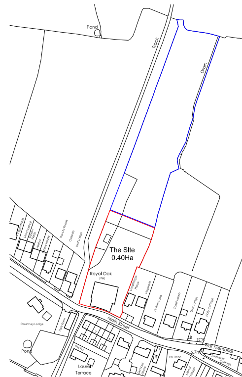
Location Plan 1:1250
